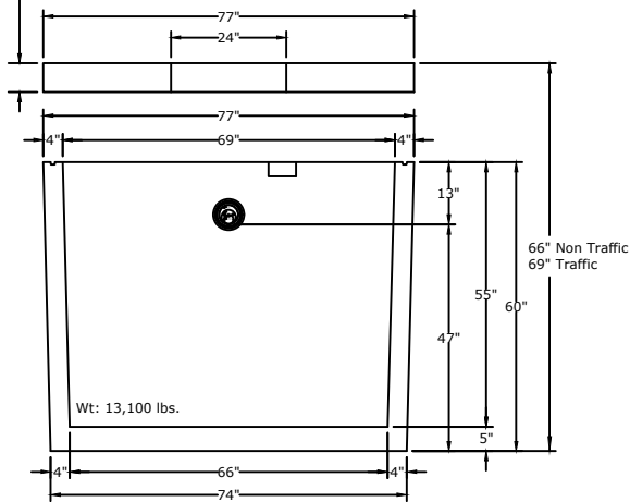
OUTLET ELEVATION
