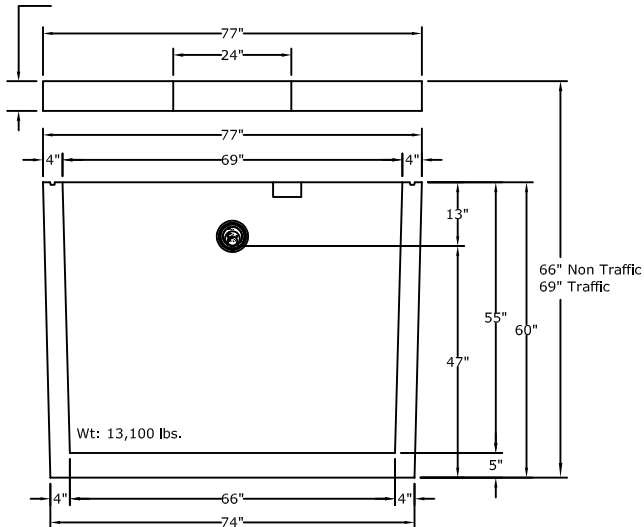
OUTLET ELEVATION
