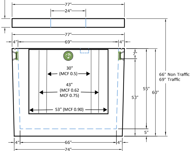
INLET ELEVATION
