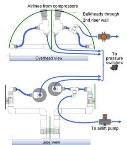
PHOTO 15 DOUBLE COMPRESSOR AIRLINE PLUMBING
