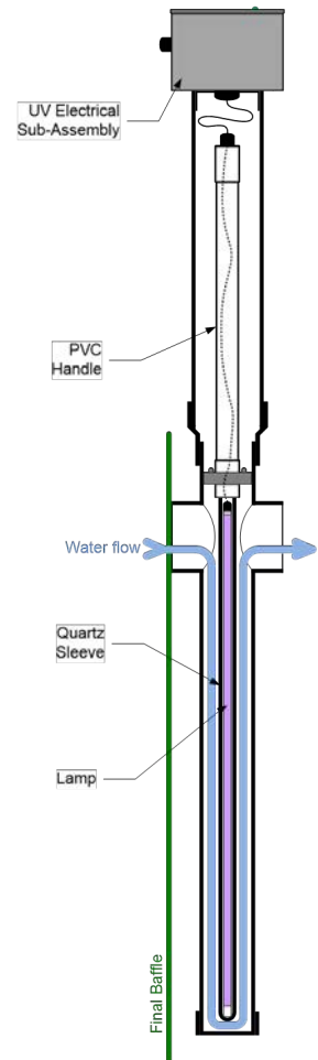
PHOTO 27 COMPLETE UV ASSEMBLY
