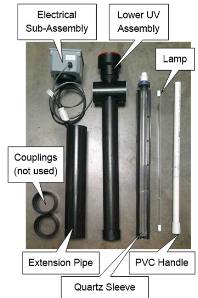
PHOTO 18 UV ASSEMBLY COMPONENTS
