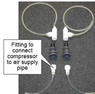
PHOTO 9 DOUBLE COMPRESSOR AIR SUPPLY ASSEMBLY
