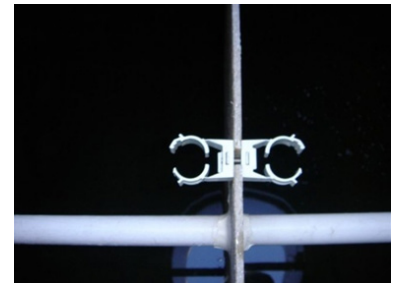
PHOTO 3 PIPE HANGER MOUNTED LOOSELY
