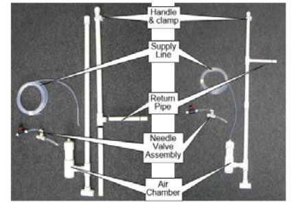
PHOTO 41 AIRLIFT RECIRCULATION PUMP ASSEMBLY
