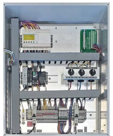
PHOTO 53 PUMPED DISCHARGE ALARM CONTROL PANEL
