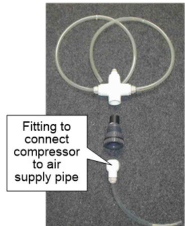
PHOTO 8 SINGLE COMPRESSOR AIR SUPPLY ASSEMBLY
