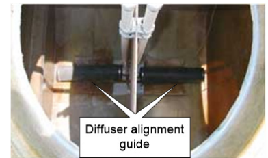
PHOTO 4 LOWER DIFFUSER ASSEMBLY MOUNTED ON PIPE HANGERS WITH DIFFUSERS IN ALIGNMENT GUIDE
