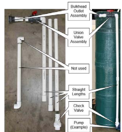
PHOTO 35 PUMP PLUMBING
