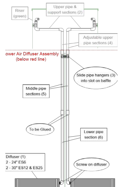
ILLUSTRATION 1 AIR DIFFUSER ASSEMBLY
