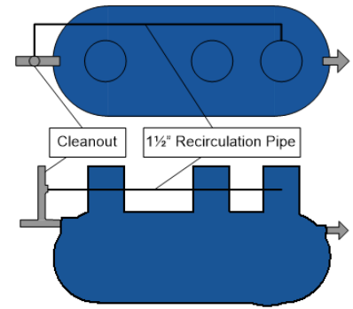
PHOTO 48 RECIRCULATION PIPE ROUTED TO THE CLEAN-OUT IN FRONT OF TANK
