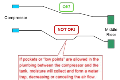
PHOTO 56 COMPRESSOR PLUMBING
