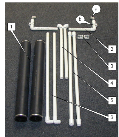
PHOTO 1 AIR DIFFUSER PARTS
