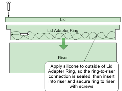
PHOTO 57 LID INSTALLATION
