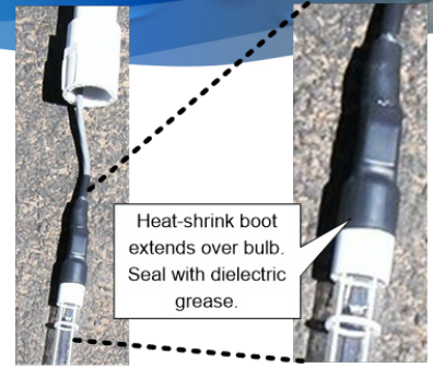
PHOTO 23 CONNECTION TO UV LAMP
