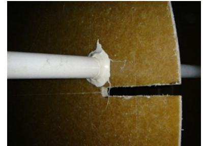
PHOTO 2 PIPE HANGER MOUNTING SLOT
