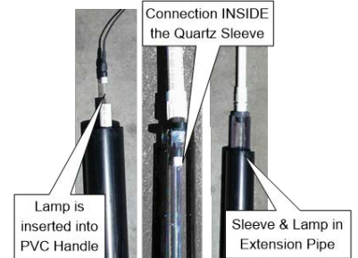
PHOTO 24 LAMP INSERTED THROUGH PVC HANDLE INTO QUARTZ SLEEVE, THEN INTO EXTENSION PIPE
